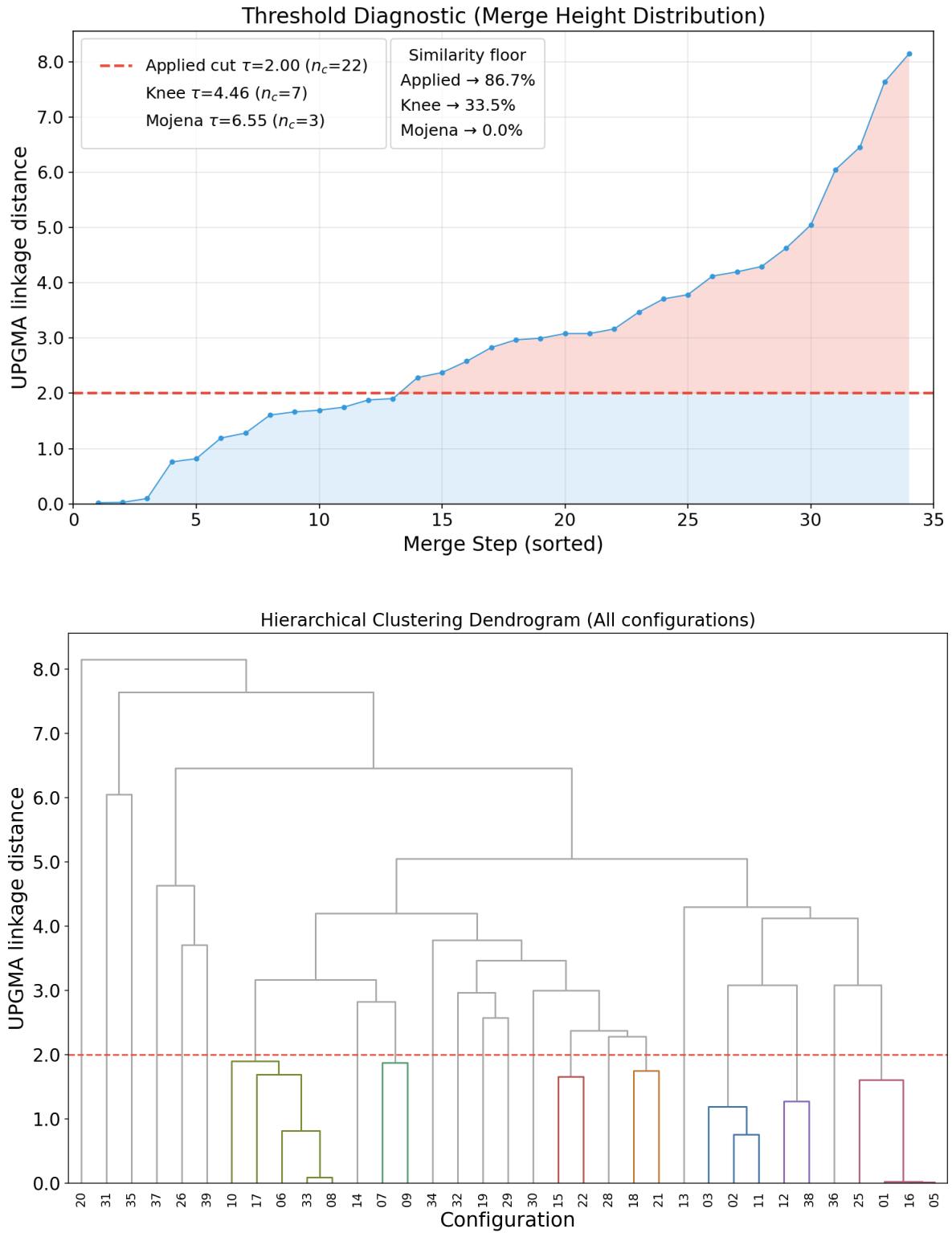
Figure 15: Final COSMIC analysis of the refined ensemble: the threshold diagnostic used \tau = 2.0 and the dendrogram grouping all refined structures into 22 unique motifs.
