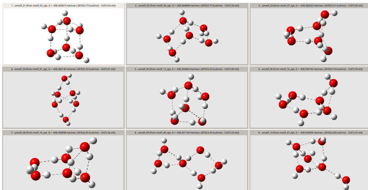
Figure 28: Subset of unique motifs identified for (\text{H}_2\text{O})_6 system via the Two Step protocol.
