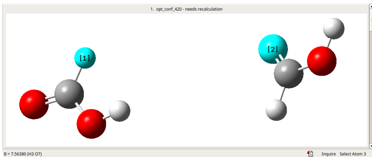
Figure 34: A dissociated arrangement ( r > 7.5 Å) of the kind flagged as critical when it cannot be recovered; such structures are excluded from the final ensemble.
