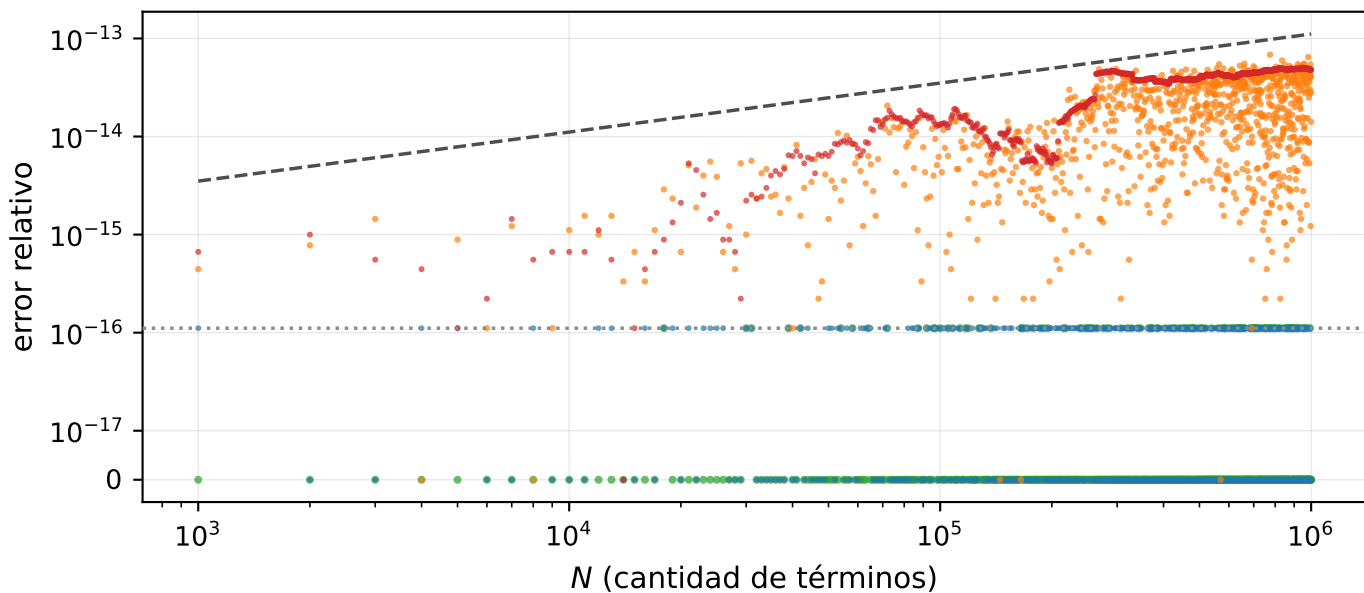
(b) N = 1000, 2000, \dots, 10^6
