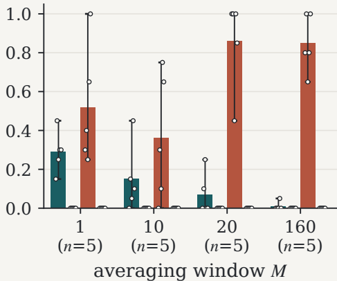
fraction converged
