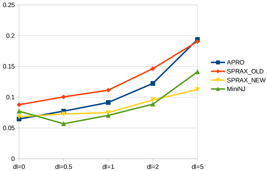
Error by DL rate
