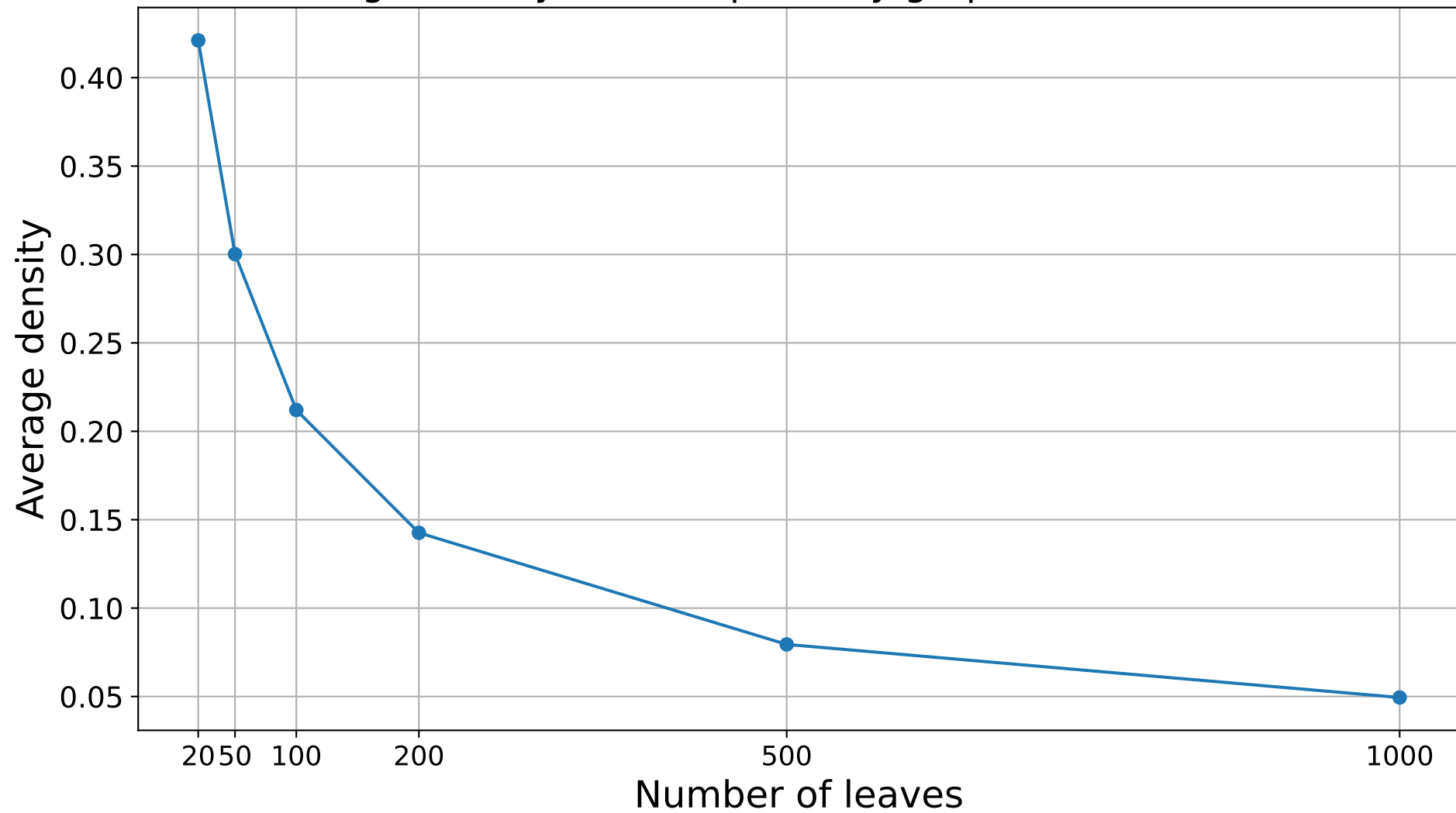
Average density of incompatibility graphs of random trees
