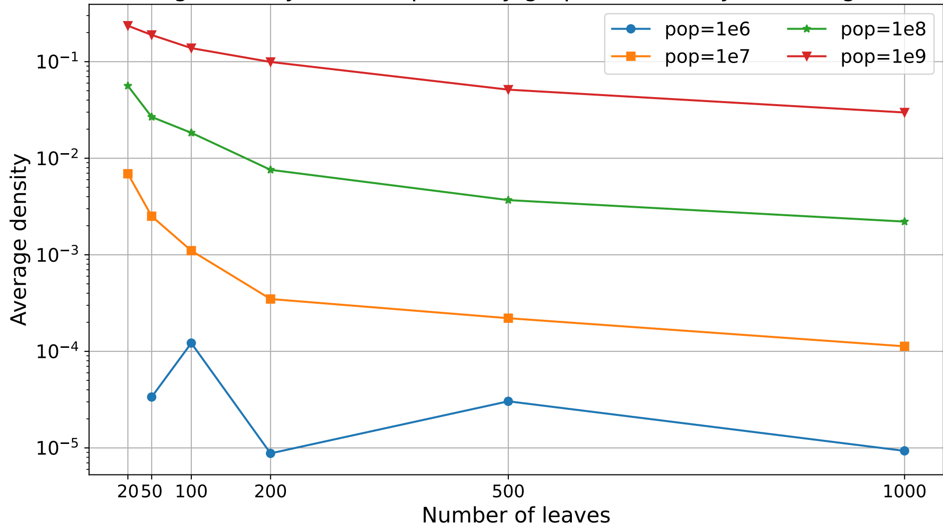
Average density of incompatibility graphs of SimPhy trees (logscale)
