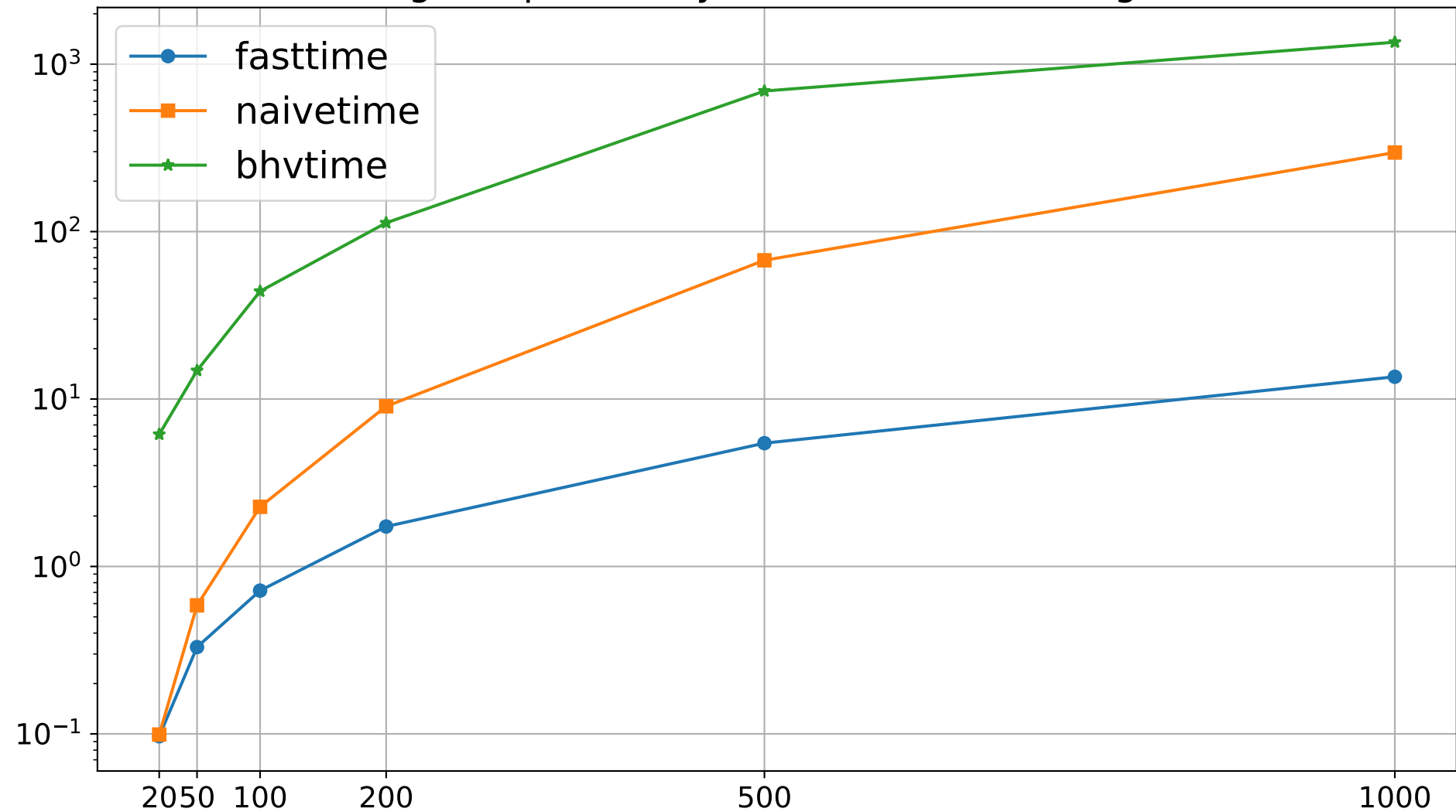
Timing comparison by number of leaves (logscale)
