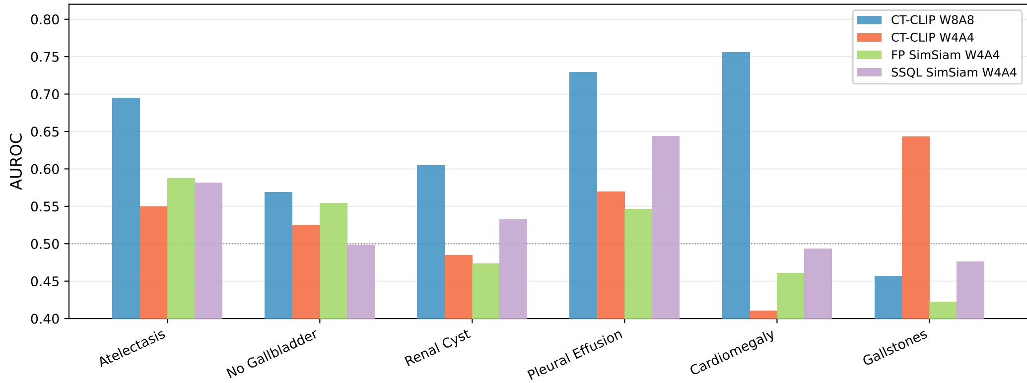
Quantized AUROC per condition — W8A8 and W4A4 (N = max per condition)
