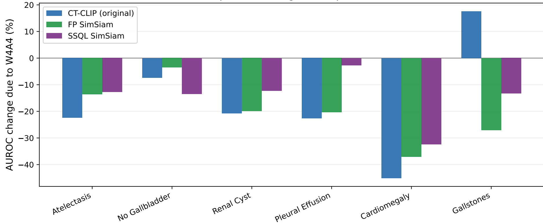
W4A4 quantization degradation per condition
