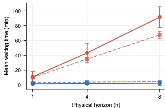
b Waiting-time growth under load
