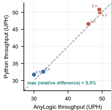
d Cross-platform throughput trend consistency
