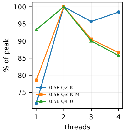
Pi 5 (4 identical A76)
