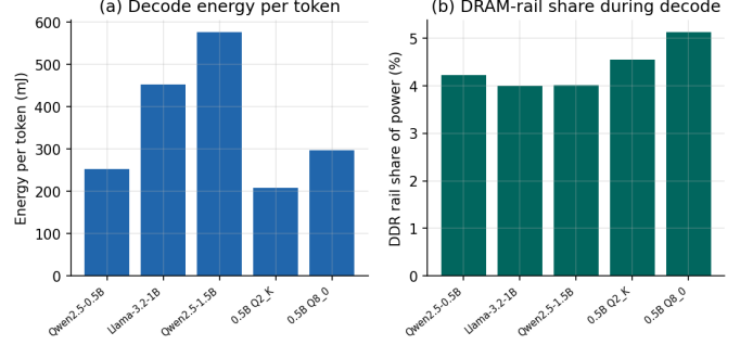
Fig. 4. (a) Energy per decoded token (PMIC), rising with model size. (b) The DRAM rail is only 4% to 5% of package power: the memory-wall energy is paid as core stalls, not DRAM-interface power.
