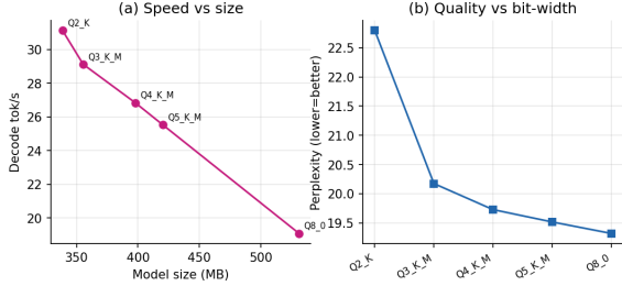
Fig. 3. Quantization frontier (Qwen2.5-0.5B). Lower-bit quantization moves fewer bytes per token, raising decode throughput and shrinking the footprint together.
