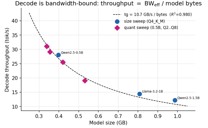
Fig. 1. Decode is bandwidth-bound. Measured decode throughput matches the roofline BW_{\text{eff}}/\text{model bytes} (dashed) across both the parameter-size sweep (circles) and the quantization sweep (diamonds), sustaining 73–86% of the 13.98 GB/s DRAM peak ( R^2 = 0.98 over all 7 points). Fewer bytes—from fewer params or fewer bits—means proportionally faster decode.
