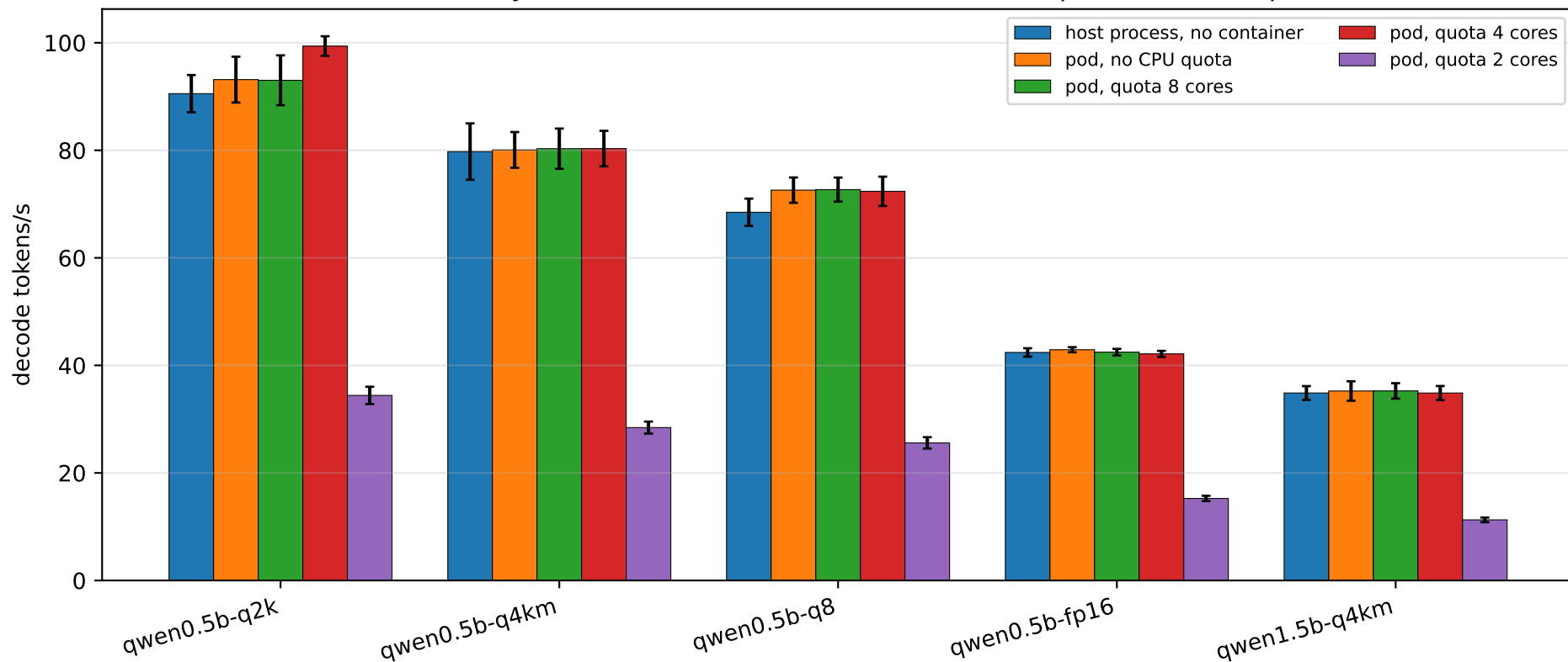
Same binary, same model file, same machine: host process versus pod
