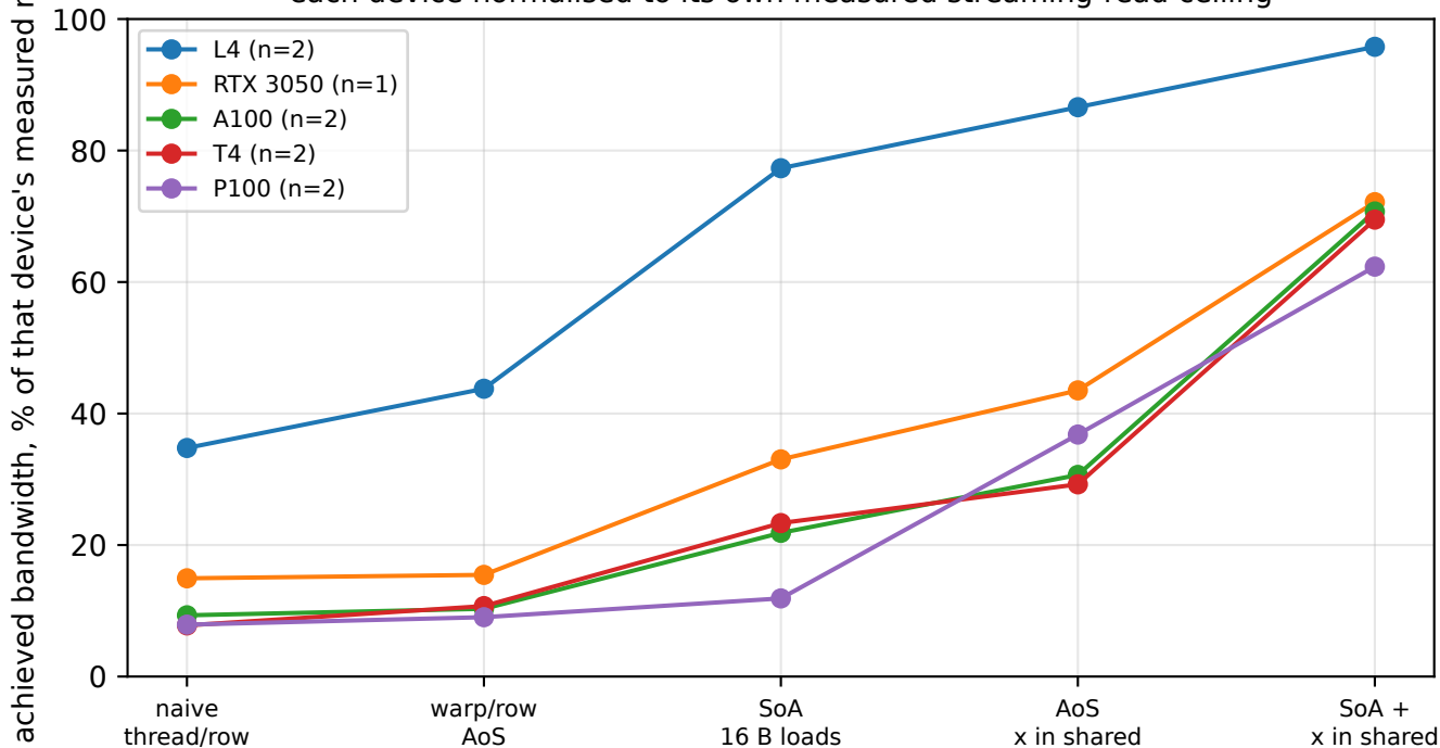
Quantized GEMV optimisation ladder, q8_0, 11008-98304 x 4096 each device normalised to its own measured streaming-read ceiling
