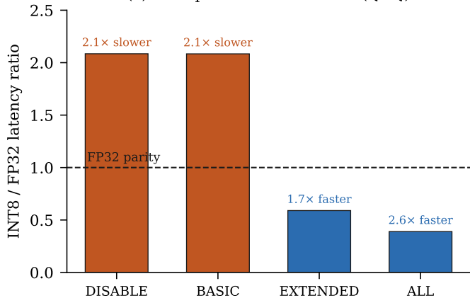
(a) The optimization-level cliff (QDQ)
