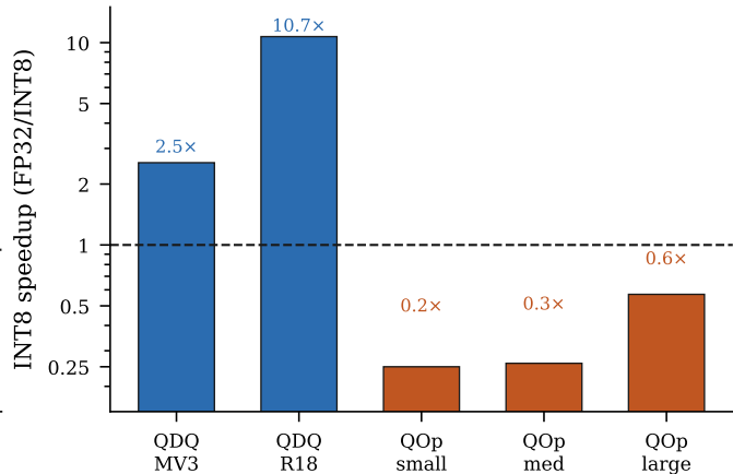
(b) Format decides the sign (ENABLE\_ALL)
