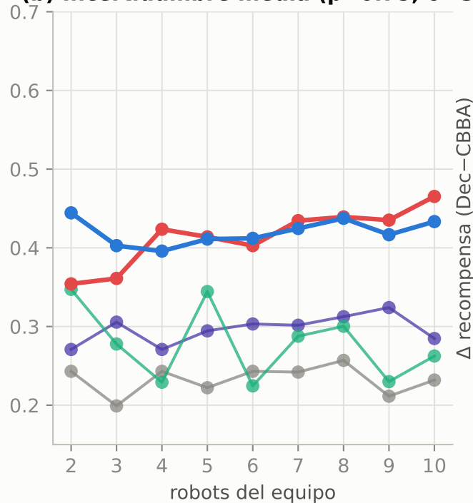
(b) Incertidumbre media ( \rho=0.75, \sigma=3 )
