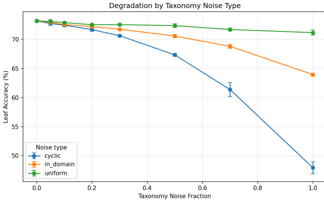
Fig. 1. Leaf-accuracy degradation by taxonomy noise type. Error bars show standard deviation across three seeds.
