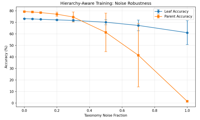
Fig. 2. Overall degradation across all hierarchy-noise rows. Parent accuracy collapses as parent supervision becomes corrupted; leaf accuracy is more robust but still degrades under structured noise.
