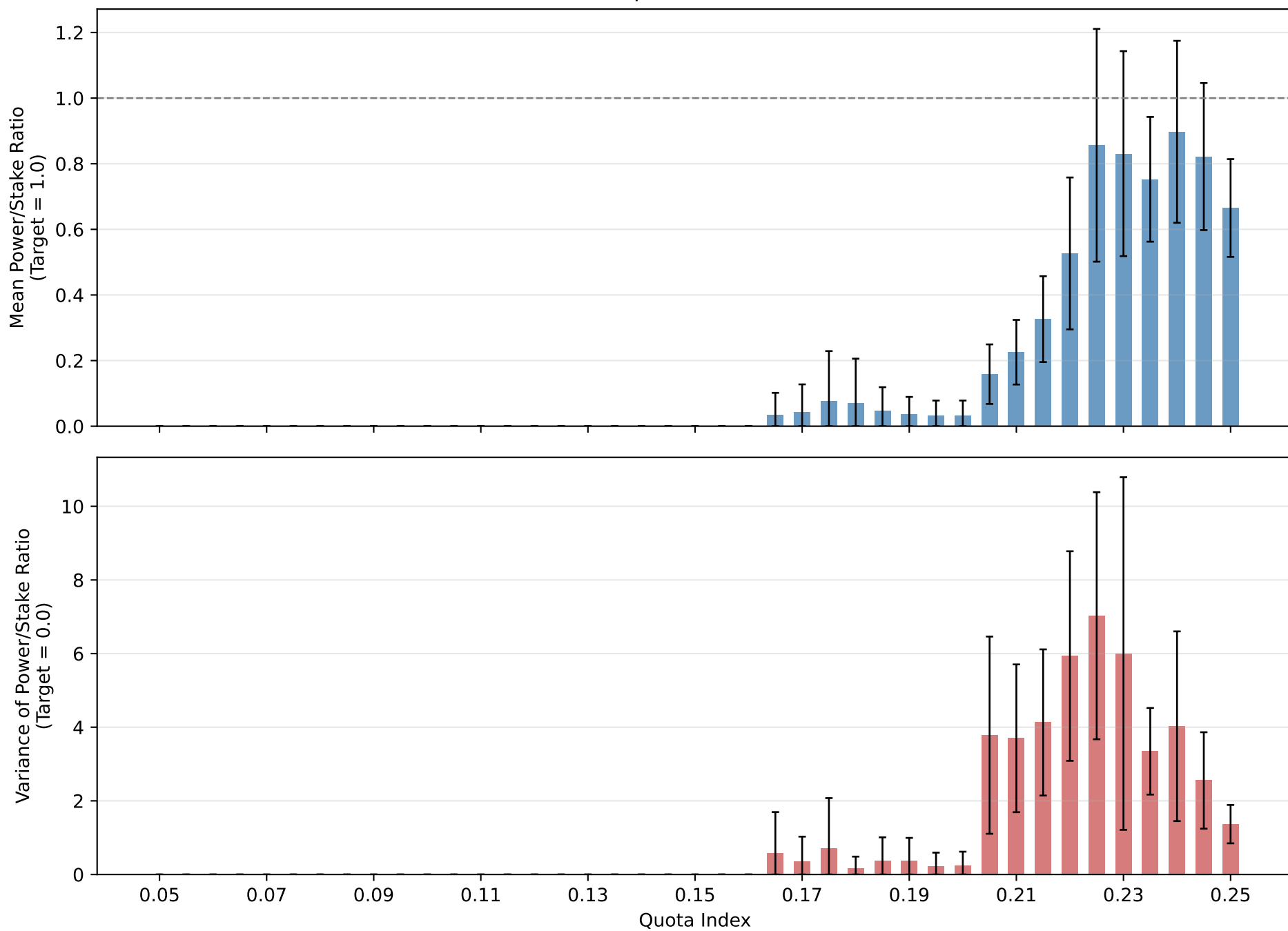
Fairness Summary by Quota (n=100) Gamma(Shape \alpha=1.0 , Scale \theta=0.5 )
