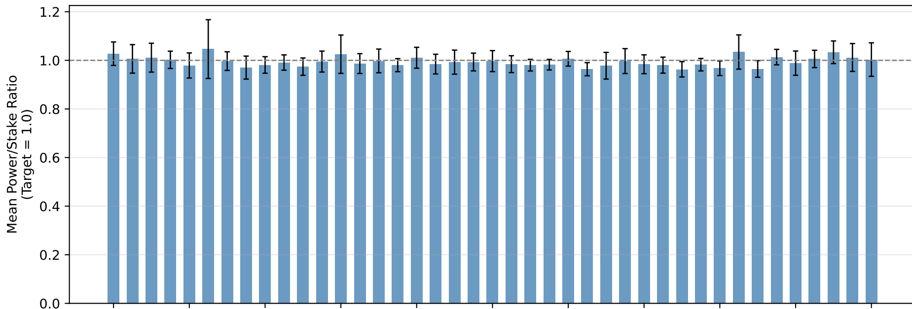
Fairness Summary by Quota (n=100) Gamma(Shape \alpha=0.5 , Scale \theta=2.0 )
