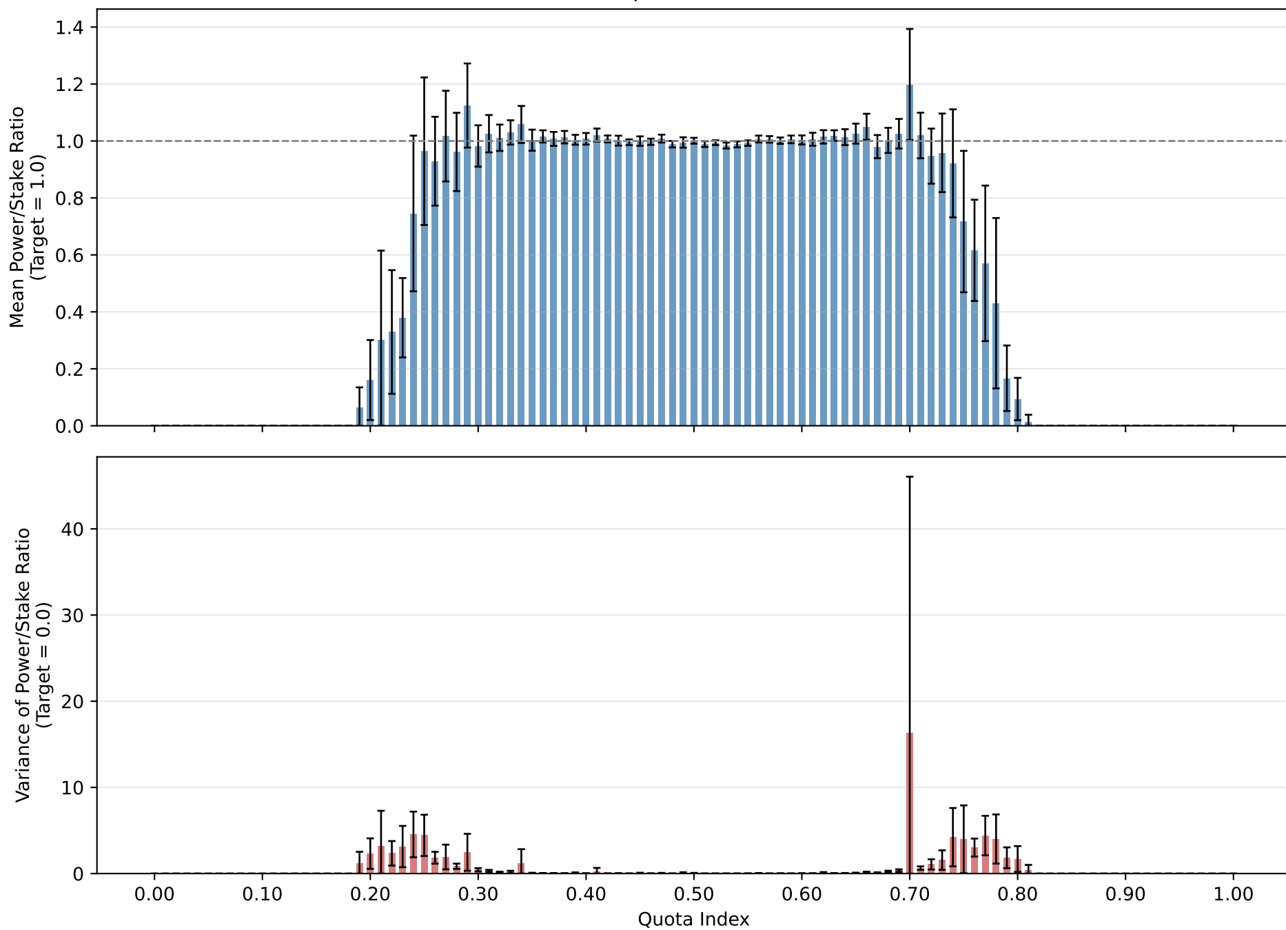
Fairness Summary by Quota (n=100) Gamma(Shape \alpha=1.0 , Scale \theta=1.0 )
