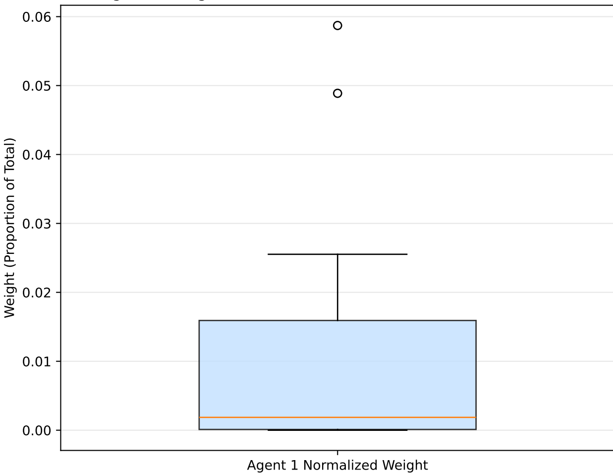
Agent 1 Weight Distribution (Gamma \alpha=0.24 , \theta=330235.0 )
