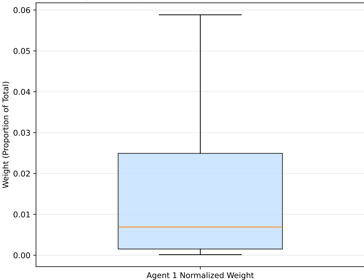
Agent 1 Weight Distribution (Gamma \alpha=0.5 , \theta=1.0 )
