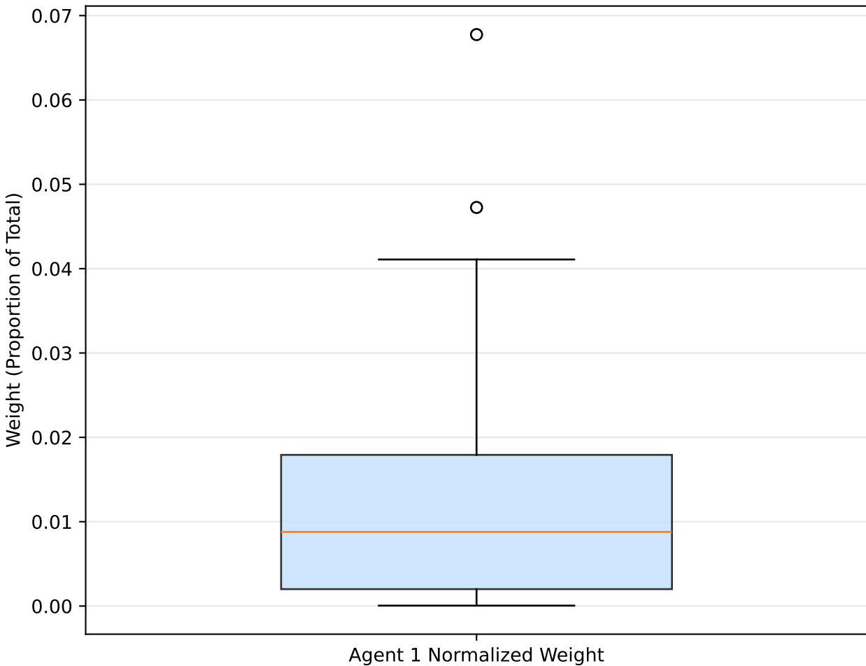
Agent 1 Weight Distribution (Gamma \alpha=0.5 , \theta=2.0 )
