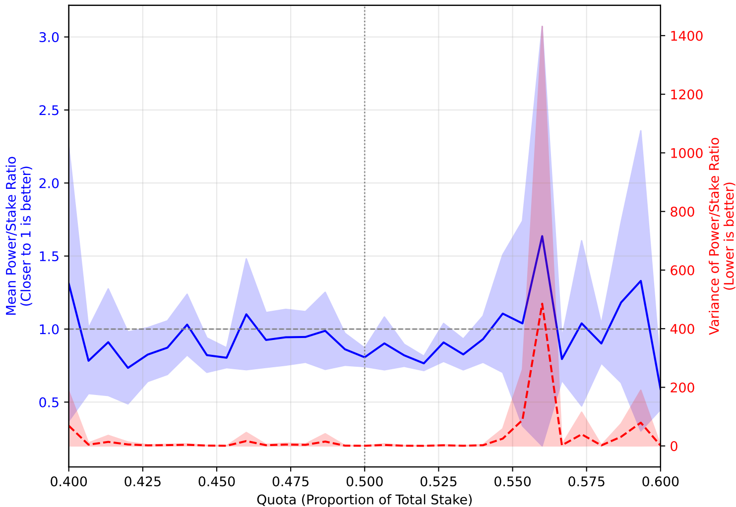
Fairness Analysis: Power vs. Stake Gamma Dist (Shape \alpha=0.24 , Scale \theta=330235.0 , n=1000 )
