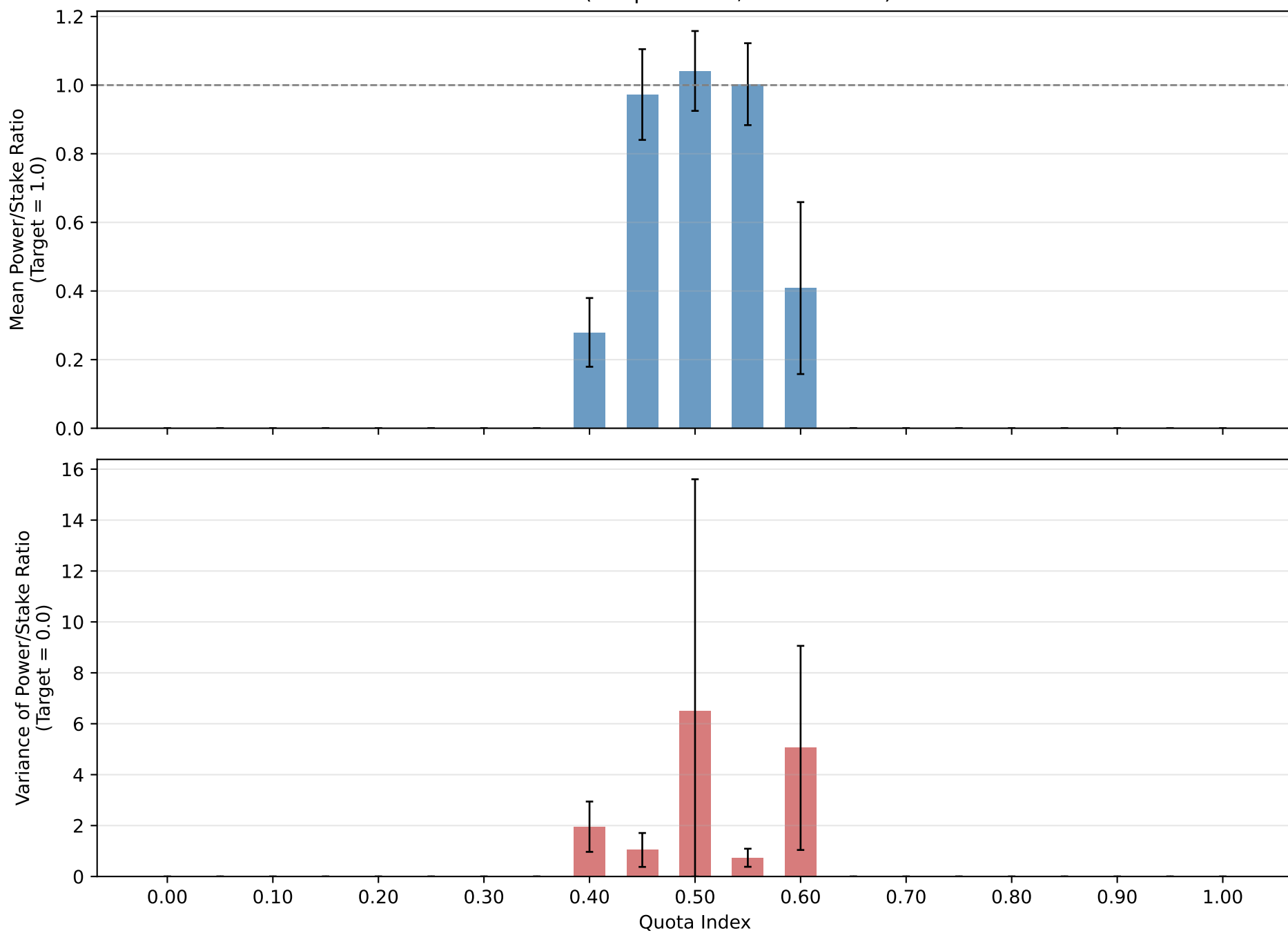
Fairness Summary by Quota (n=1000) Gamma(Shape \alpha=0.5 , Scale \theta=0.5 )
