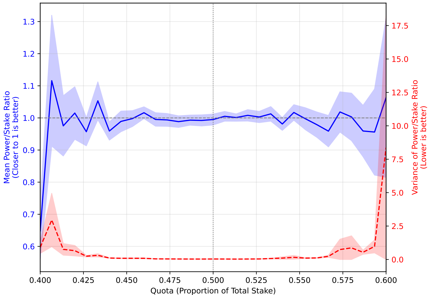
Fairness Analysis: Power vs. Stake Gamma Dist (Shape \alpha=1.0 , Scale \theta=0.5 , n=500 )
