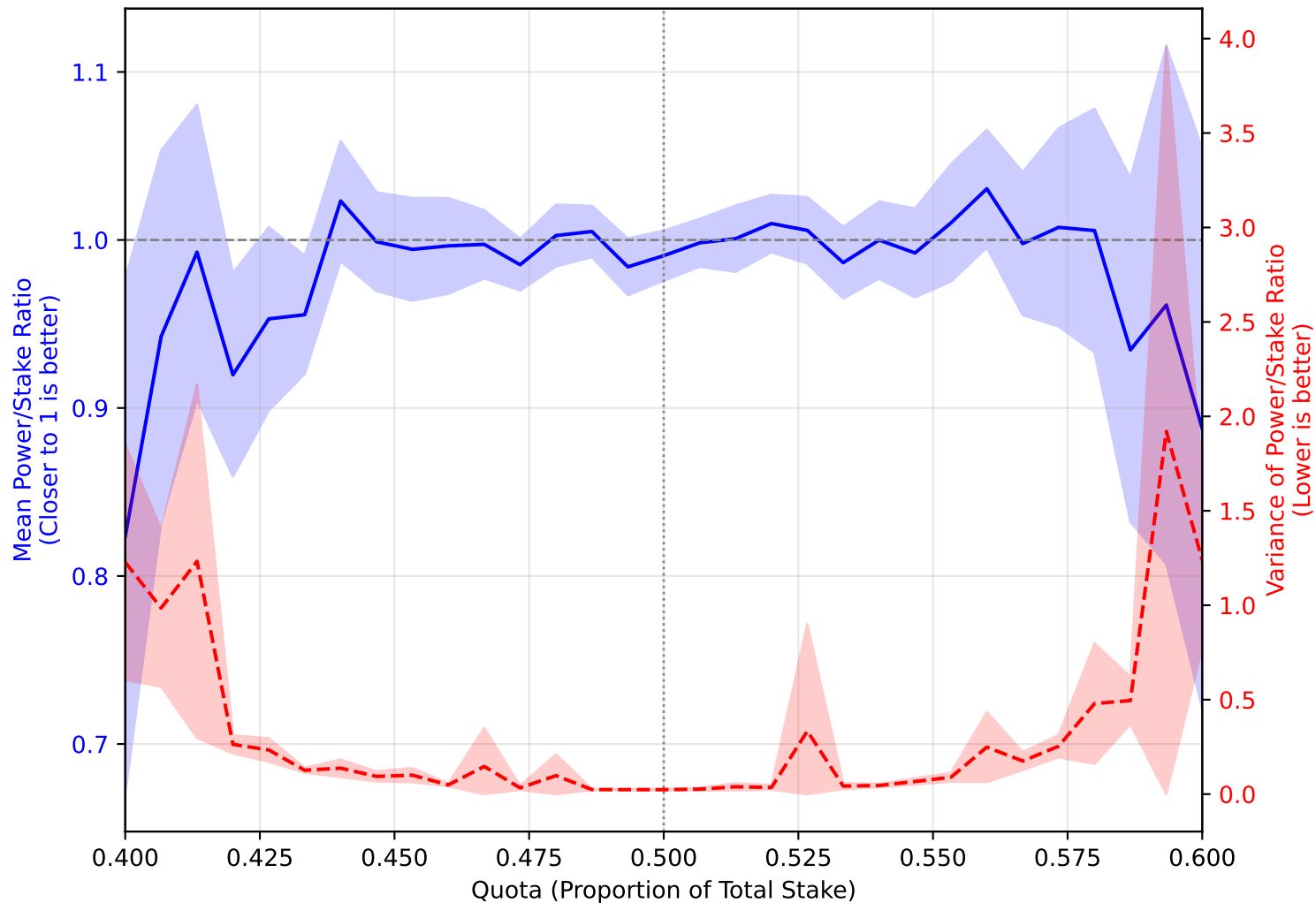
Fairness Analysis: Power vs. Stake Gamma Dist (Shape \alpha=1.0 , Scale \theta=1.0 , n=500 )
