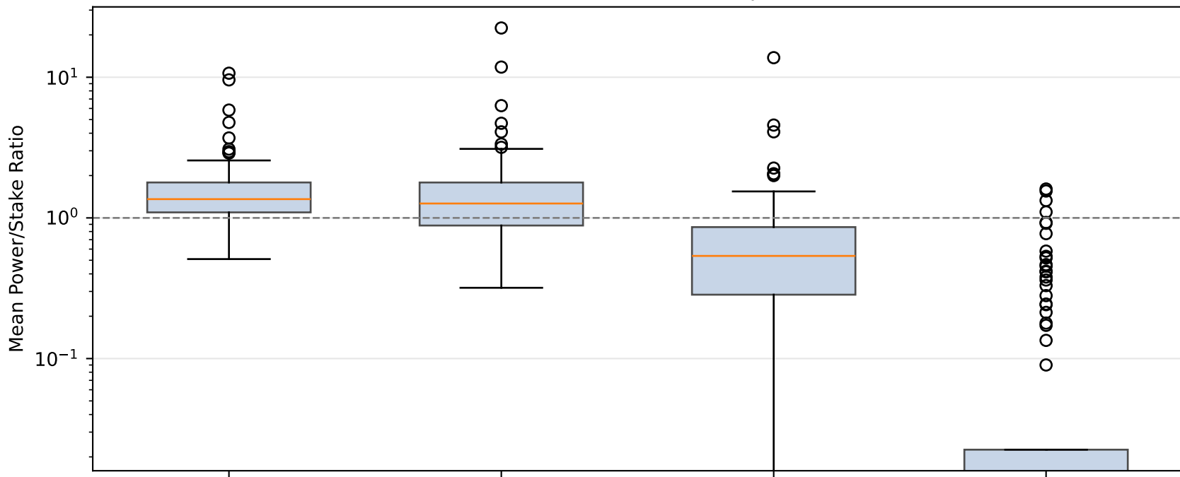
Intergroup Variance at Fixed Quota
