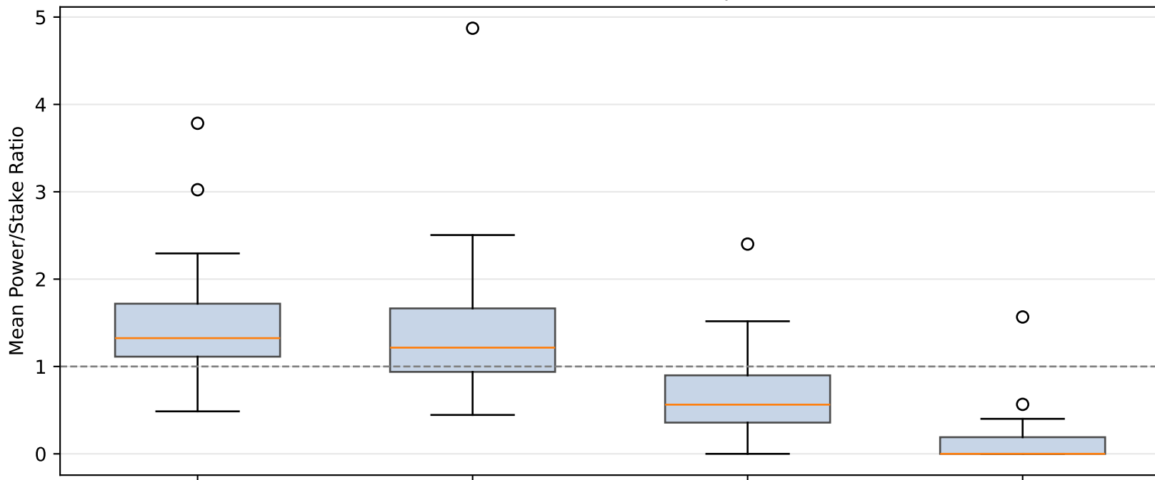
Intergroup Variance at Fixed Quota
