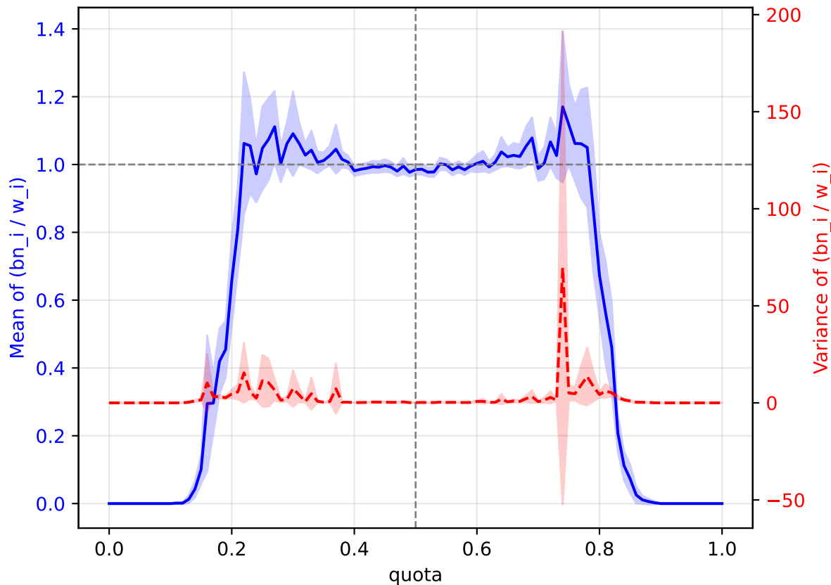
Gamma( \alpha=0.5 , \theta=1.0 ) — normalized Banzhaf ratios
