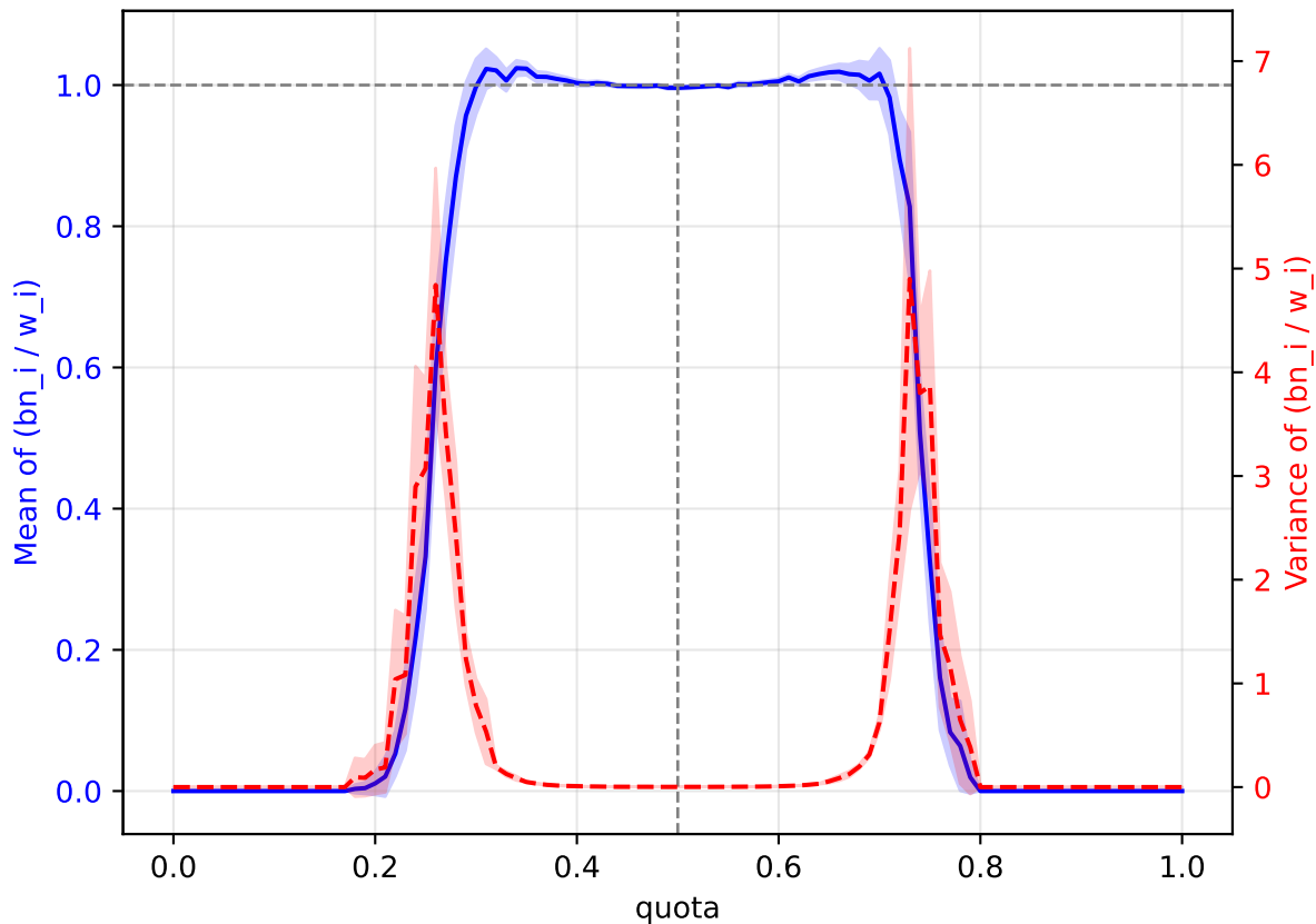
Gamma( \alpha=2.0 , \theta=2.0 ) — normalized Banzhaf ratios
