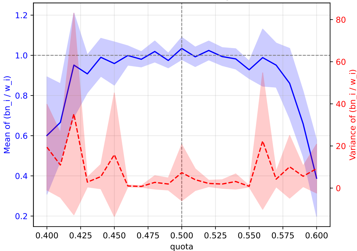
Gamma( \alpha=0.5 , \theta=0.5 ) — large n=1000
