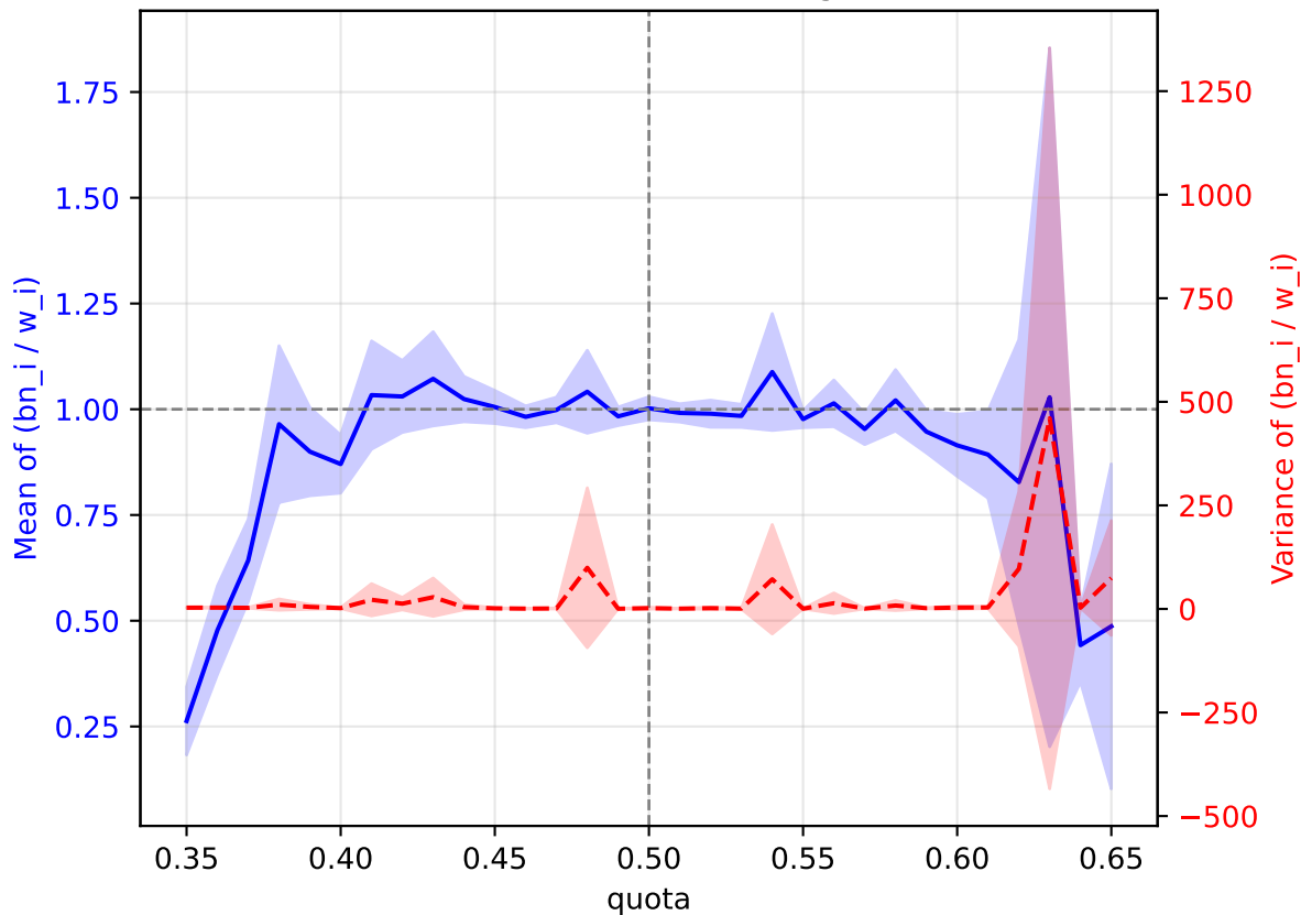
Gamma( \alpha=0.5 , \theta=0.5 ) — large n=500
