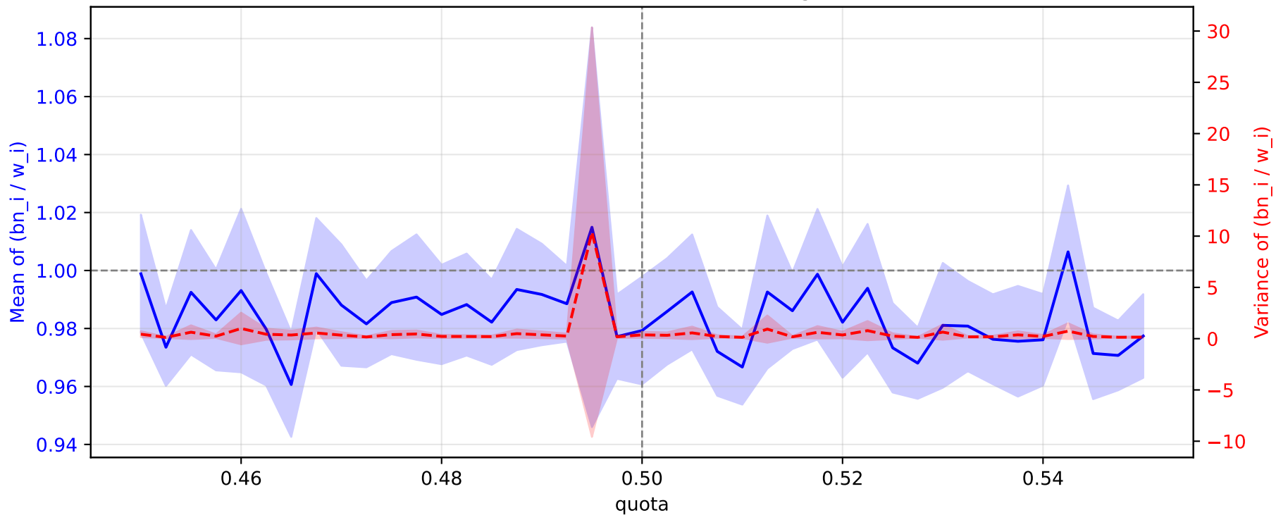
Gamma( \alpha=0.5 , \theta=0.5 ) — ratios and weight variance
