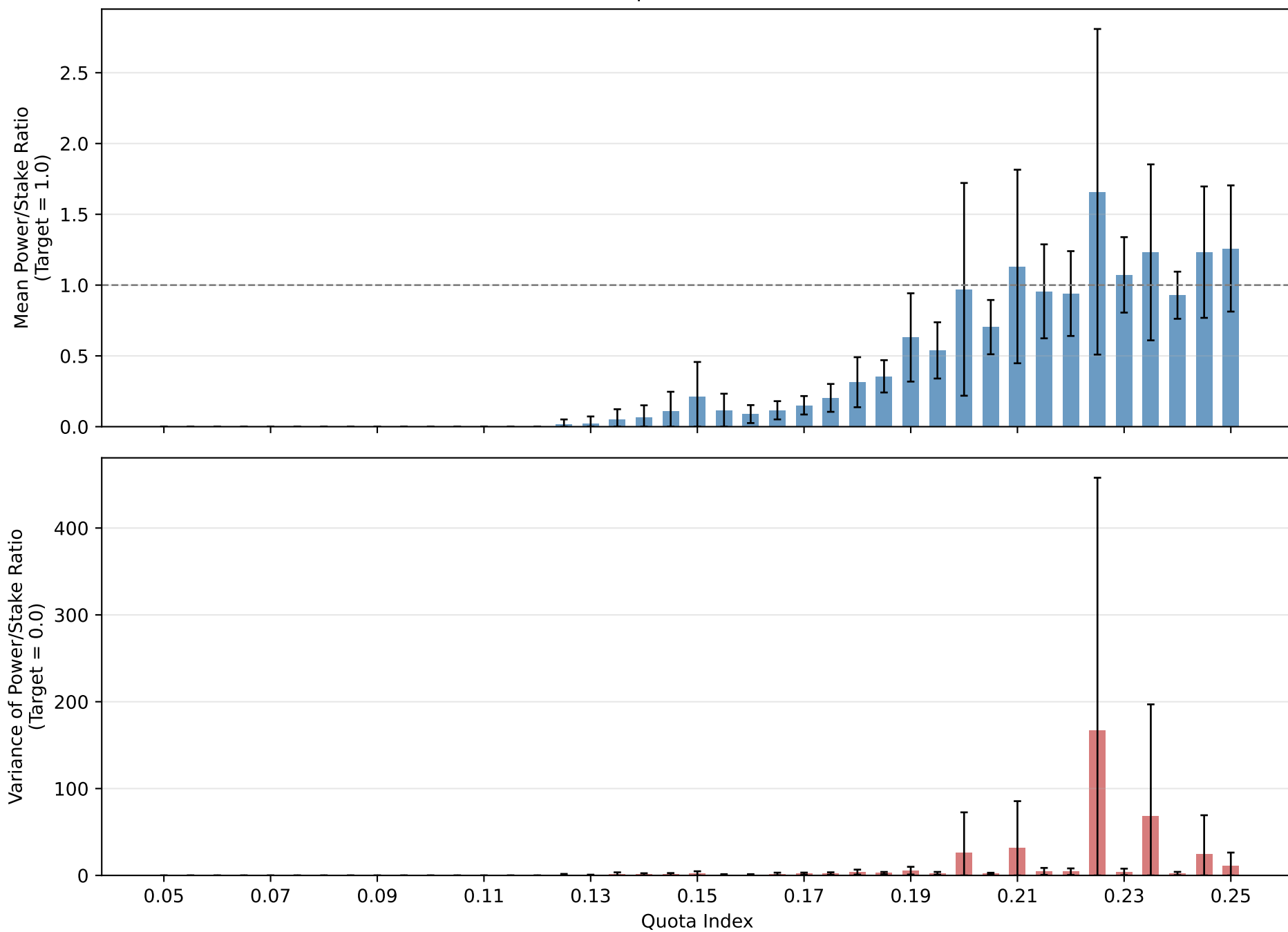
Fairness Summary by Quota (n=100) Gamma(Shape \alpha=0.5 , Scale \theta=2.0 )
