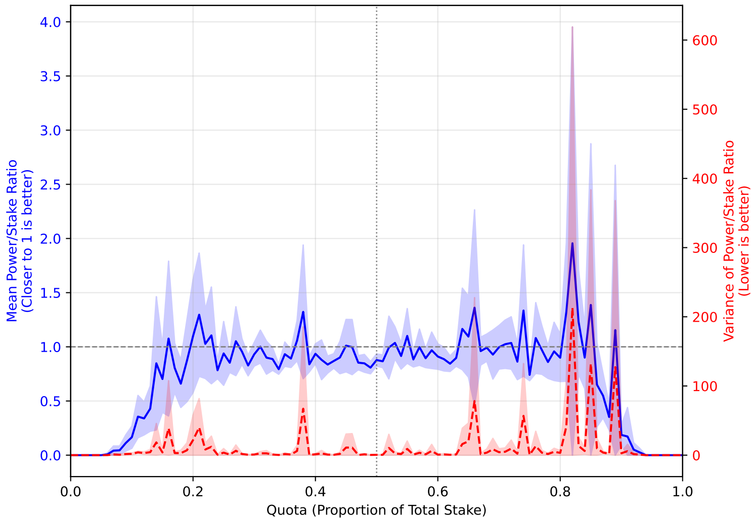
Fairness Analysis: Power vs. Stake Gamma Dist (Shape \alpha=0.24 , Scale \theta=330235.0 , n=100 )
