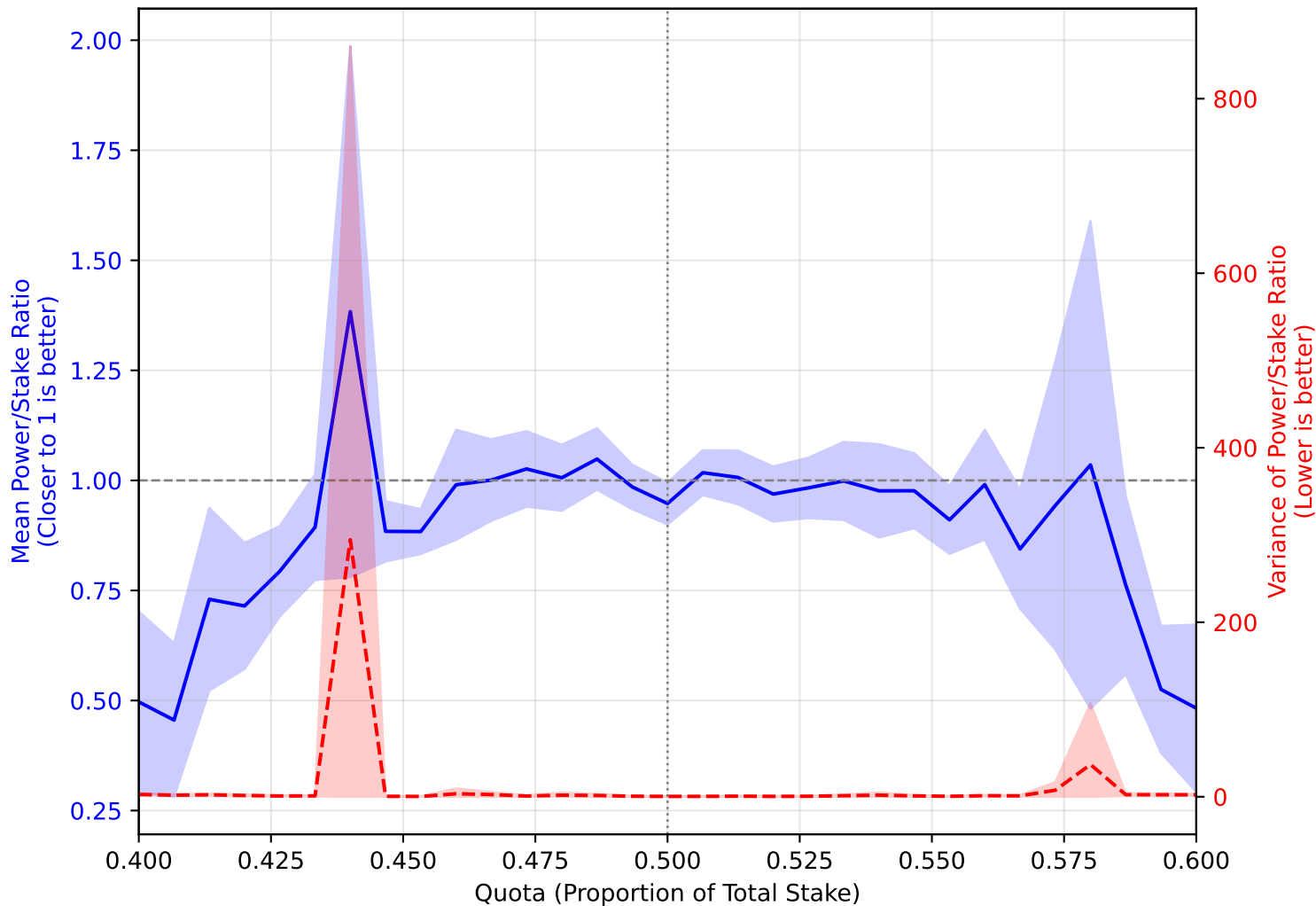
Fairness Analysis: Power vs. Stake Gamma Dist (Shape \alpha=0.5 , Scale \theta=1.0 , n=1000 )
