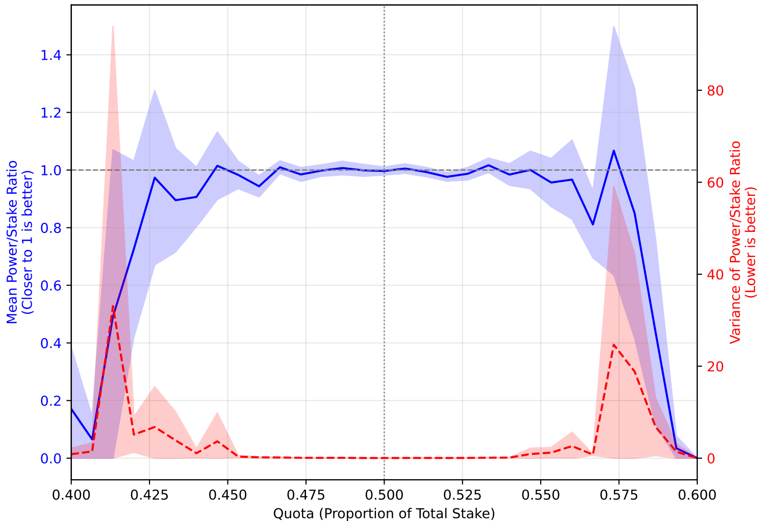
Fairness Analysis: Power vs. Stake Gamma Dist (Shape \alpha=1.0 , Scale \theta=0.5 , n=1000 )
