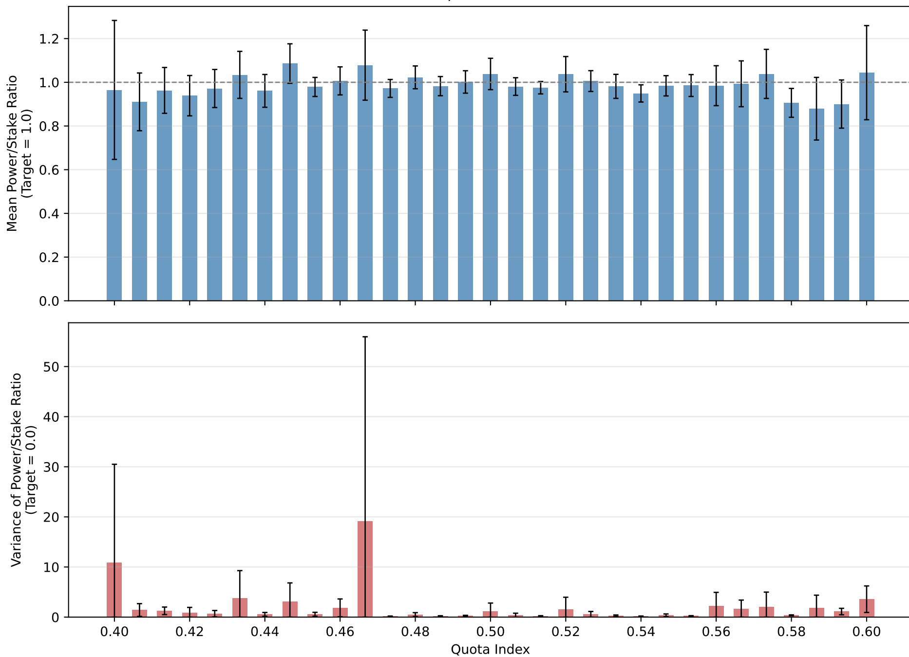
Fairness Summary by Quota (n=500) Gamma(Shape \alpha=0.5 , Scale \theta=0.5 )
