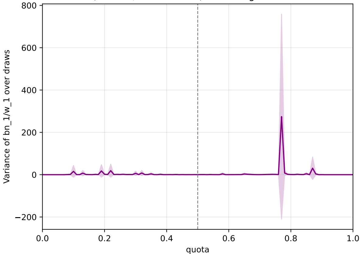
Gamma( \alpha=0.24 , \theta=330235.0 ) — First agent ratio variance
