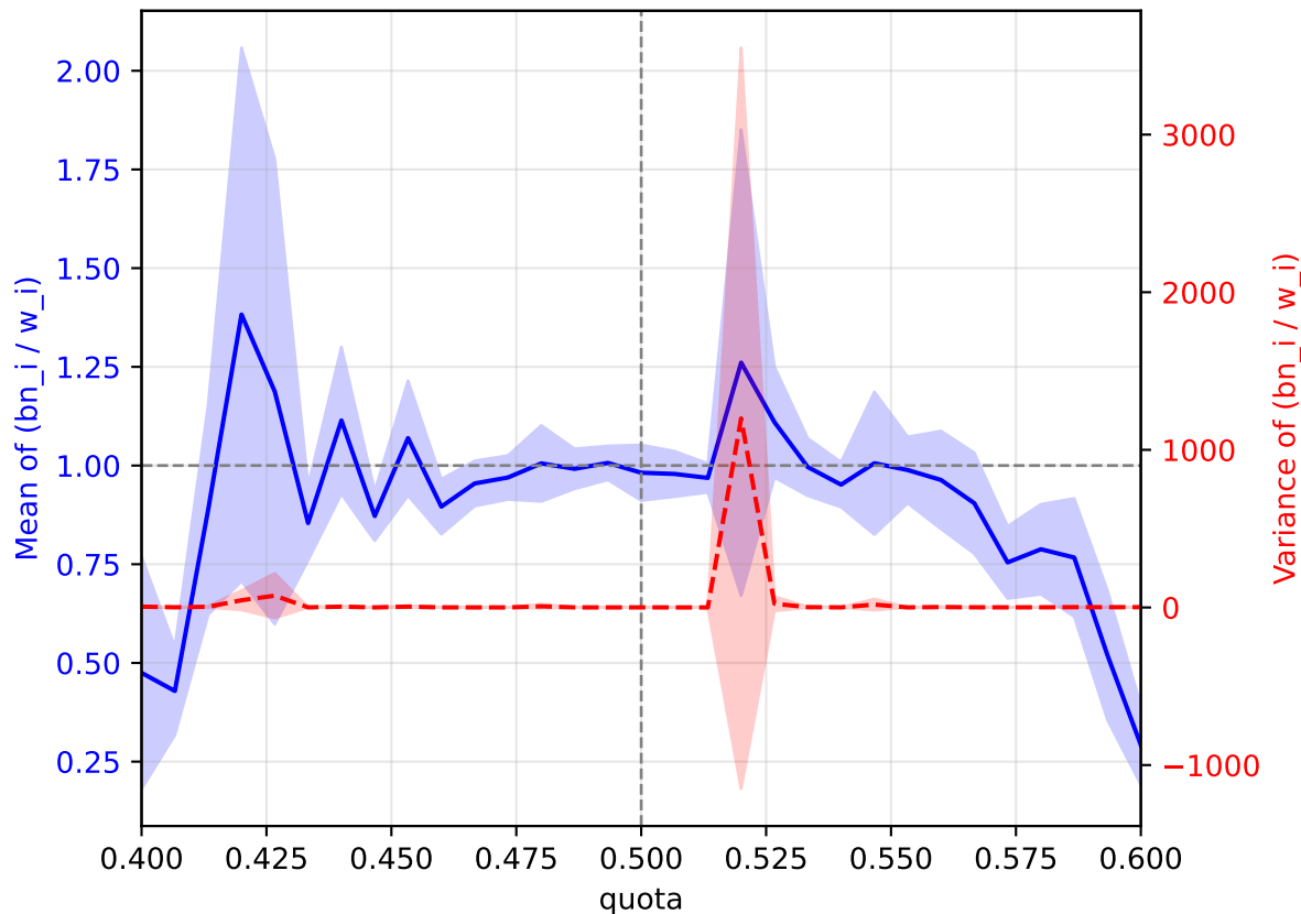
Gamma( \alpha=0.5 , \theta=0.5 ) — normalized Banzhaf ratios
