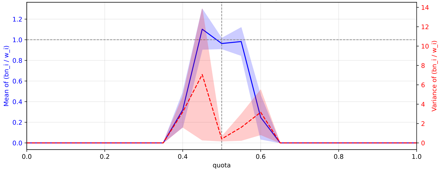
Gamma( \alpha=0.5 , \theta=0.5 ) — ratios and weight variance
