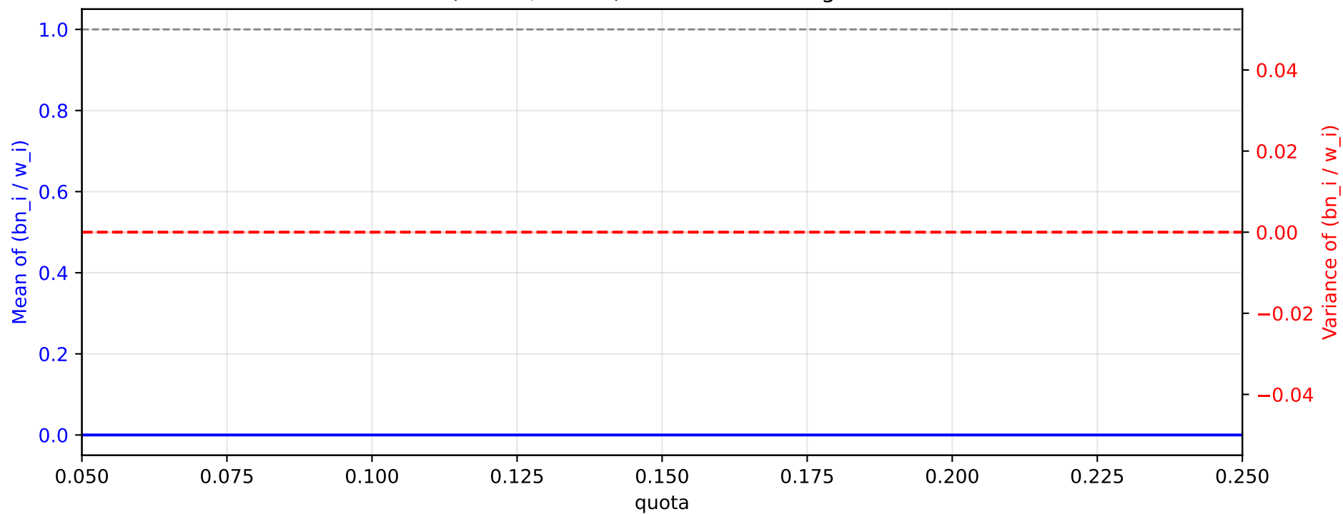
Gamma( \alpha=0.5 , \theta=1.0 ) — ratios and weight variance
