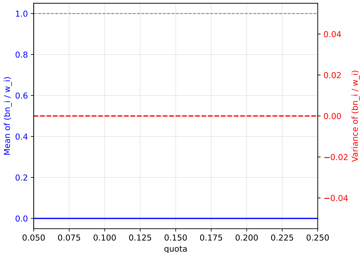
Gamma( \alpha=0.5 , \theta=2.0 ) — normalized Banzhaf ratios
