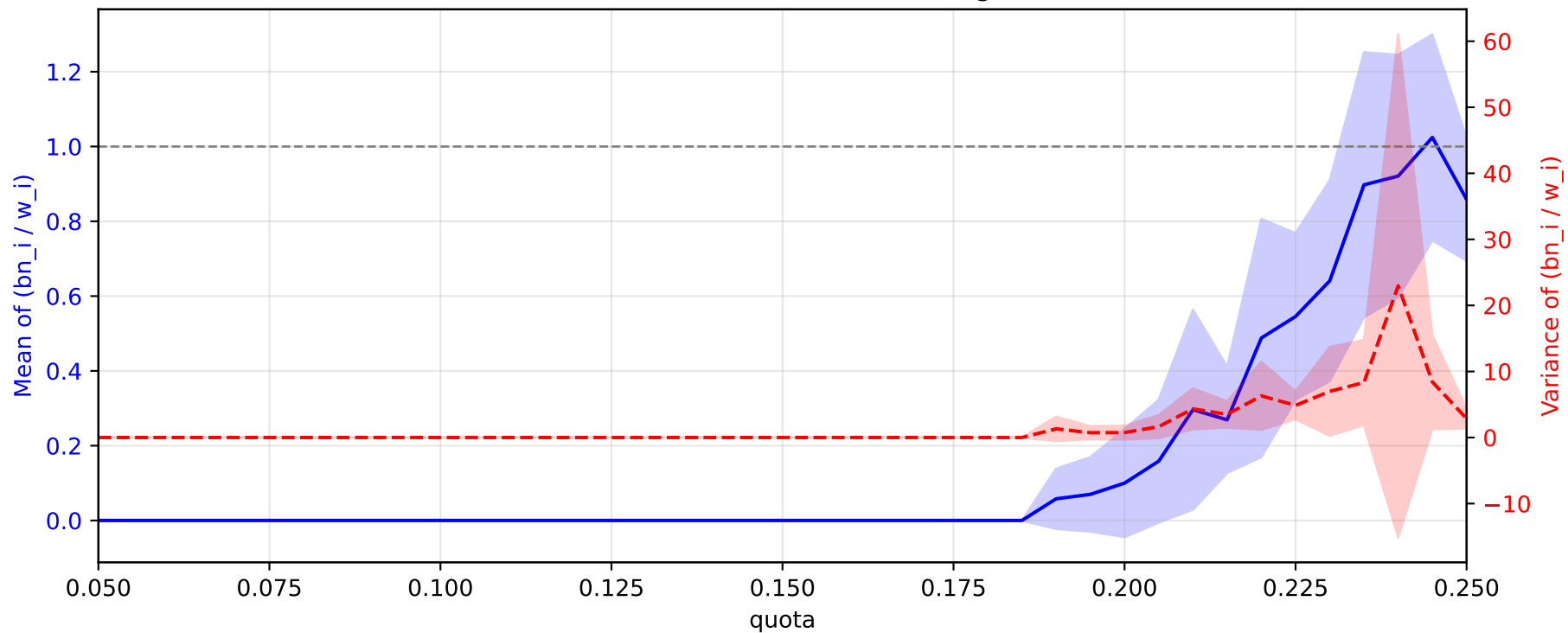
Gamma( \alpha=1.0 , \theta=0.5 ) — ratios and weight variance
