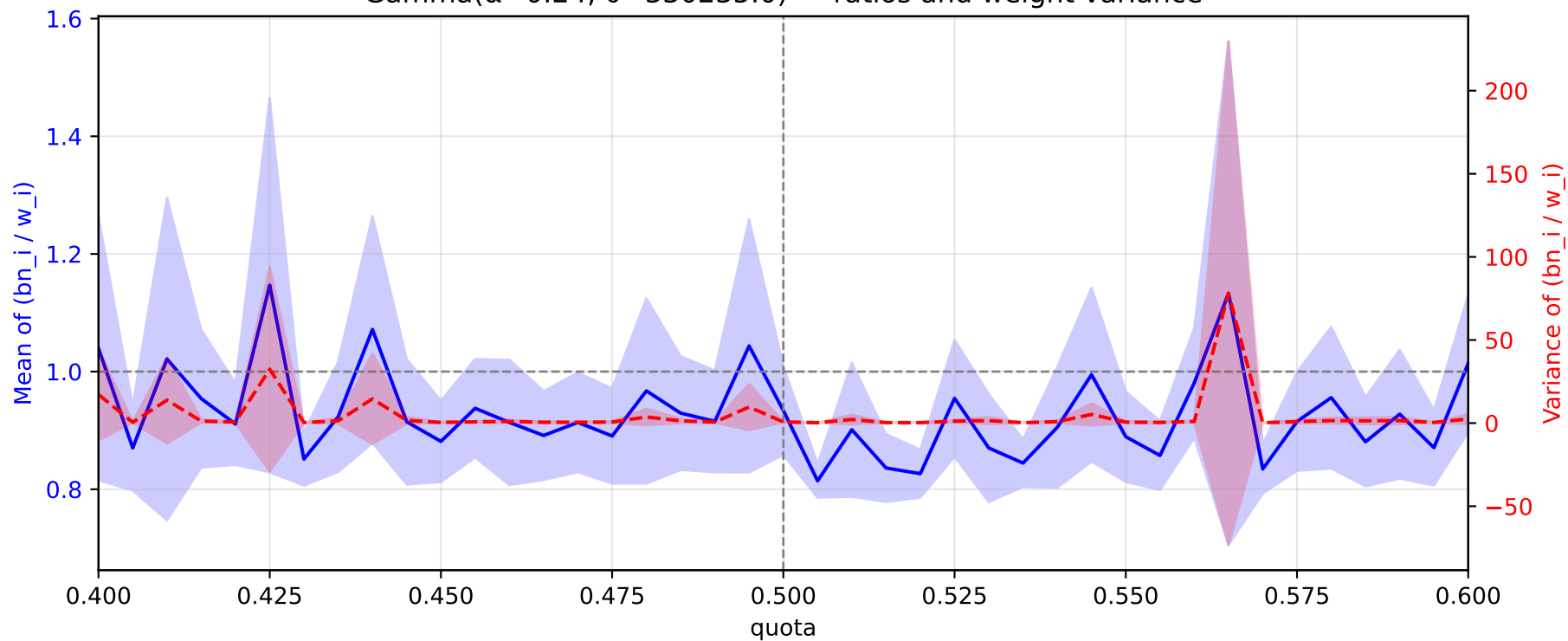
Gamma( \alpha=0.24 , \theta=330235.0 ) — ratios and weight variance
