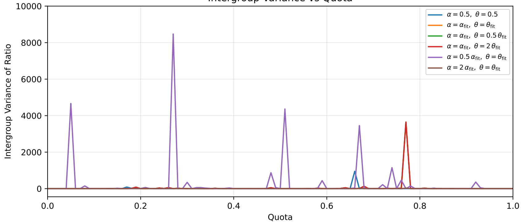
Intergroup Variance vs Quota
