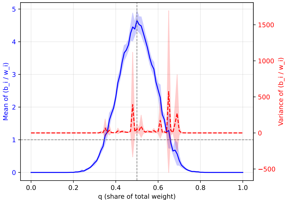
Gamma( \alpha=0.5 , \theta=1.0 ) — mean-of-means & mean-of-vars
