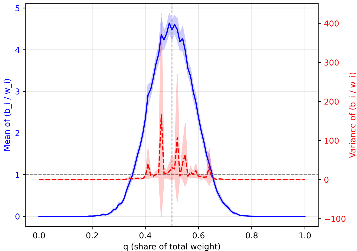
Gamma( \alpha=0.5 , \theta=2.0 ) — mean-of-means & mean-of-vars
