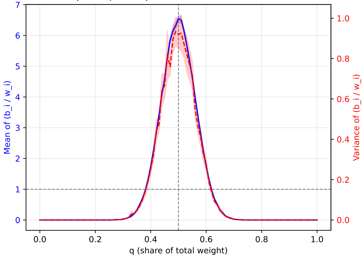
Gamma( \alpha=2.0 , \theta=0.5 ) — mean-of-means & mean-of-vars
